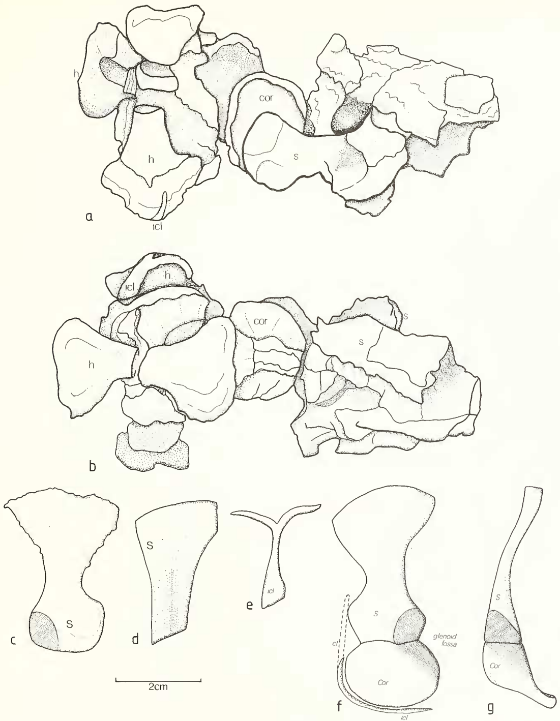
TEXT-FIG. 7. Shoulder girdle and forelimb of juvenile Scaphonyx fischeri (MCZ 1664). a, b , disarticulated shoulder girdle and forelimb elements (both scapulae, left coracoid, interclavicle, both humeri), in two views. c , right scapula in lateral view. d , partial left scapula in lateral view. e , interclavicle in ventral view. f, g , restoration of the shoulder girdle, in left lateral ( f ) and posterior ( g ) views. The clavicle is unknown.
